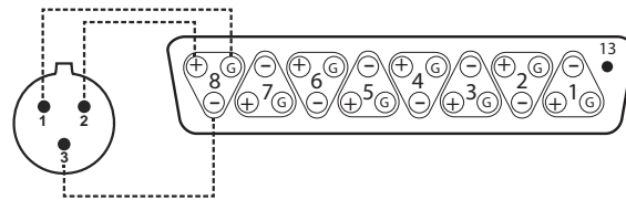
Male DB-25 Pin-out (Cable View)
